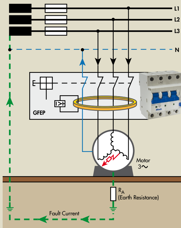
1. Ground-Fault Protection Equipment in Motor Circuit
